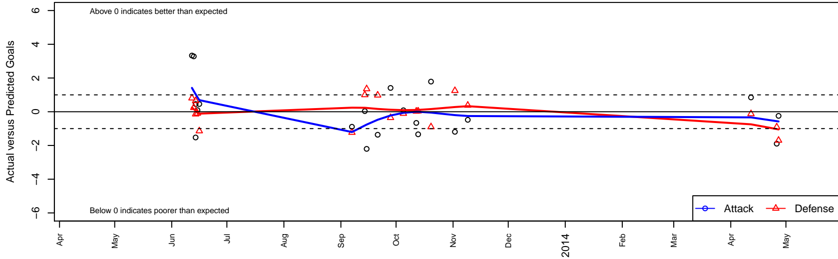
Rialto Fire SC WC B99 Dots are actual minus expected GF (blue circles) and GA (red triangles). Blue line is smoothed change in attack strength. Red is smoothed change in defense strength.
